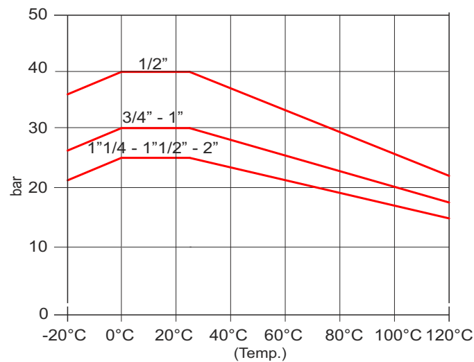
Diagramma pressione / temperatura Pressure / temperature diagram
