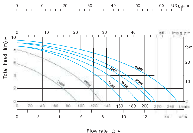
PERFORMANCE CHART AT n=2900 r/min
